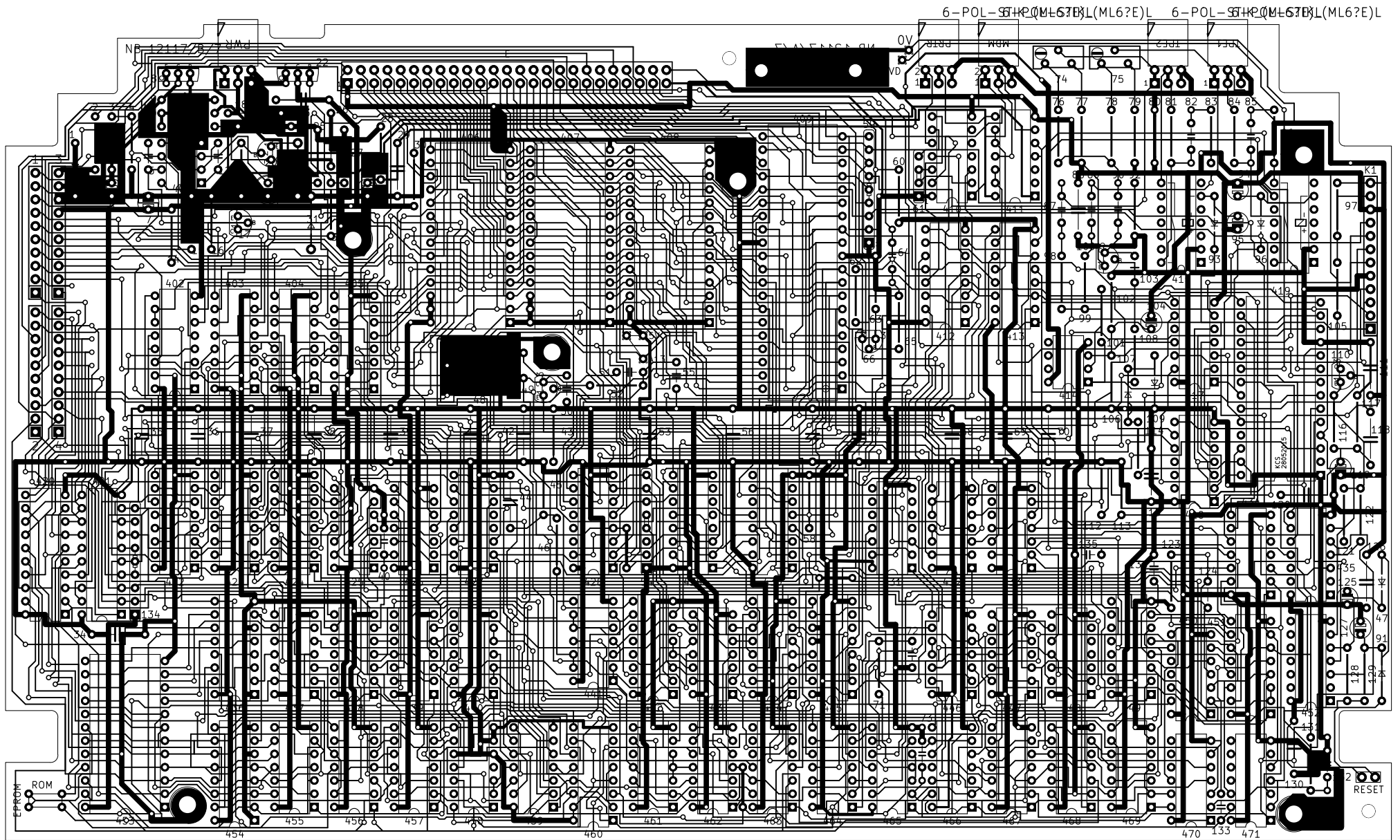
PCB from Kicad is not quite done changing it
